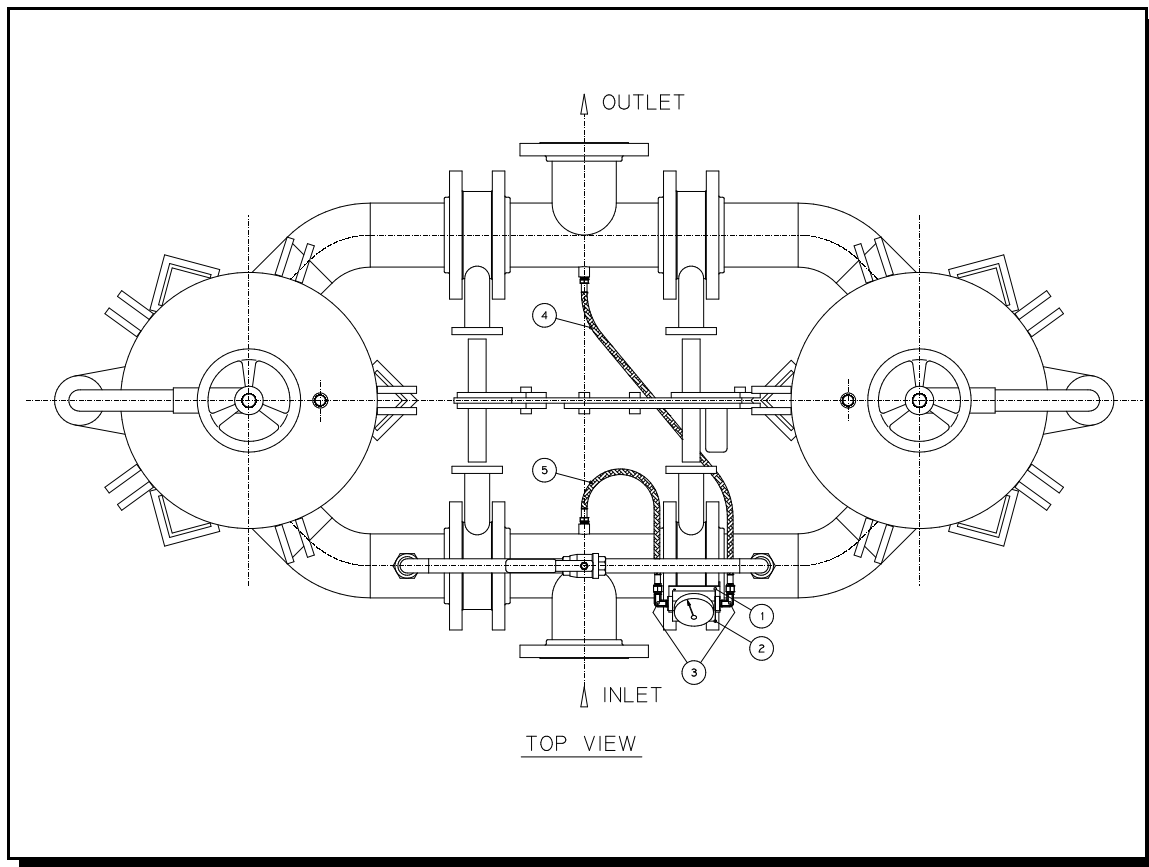
Figure 1 Typical Multi-Bag Duplex, Top View.
